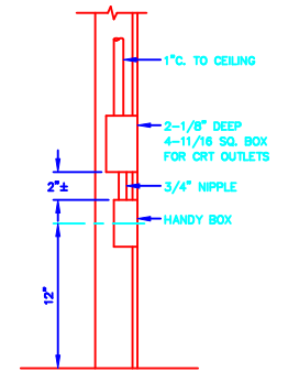
TYPICAL DETAIL CRT & TELEPHONE OUTLET AT COL. (4 CRT. & 2 TEL. CABLES) SCALE: NONE
