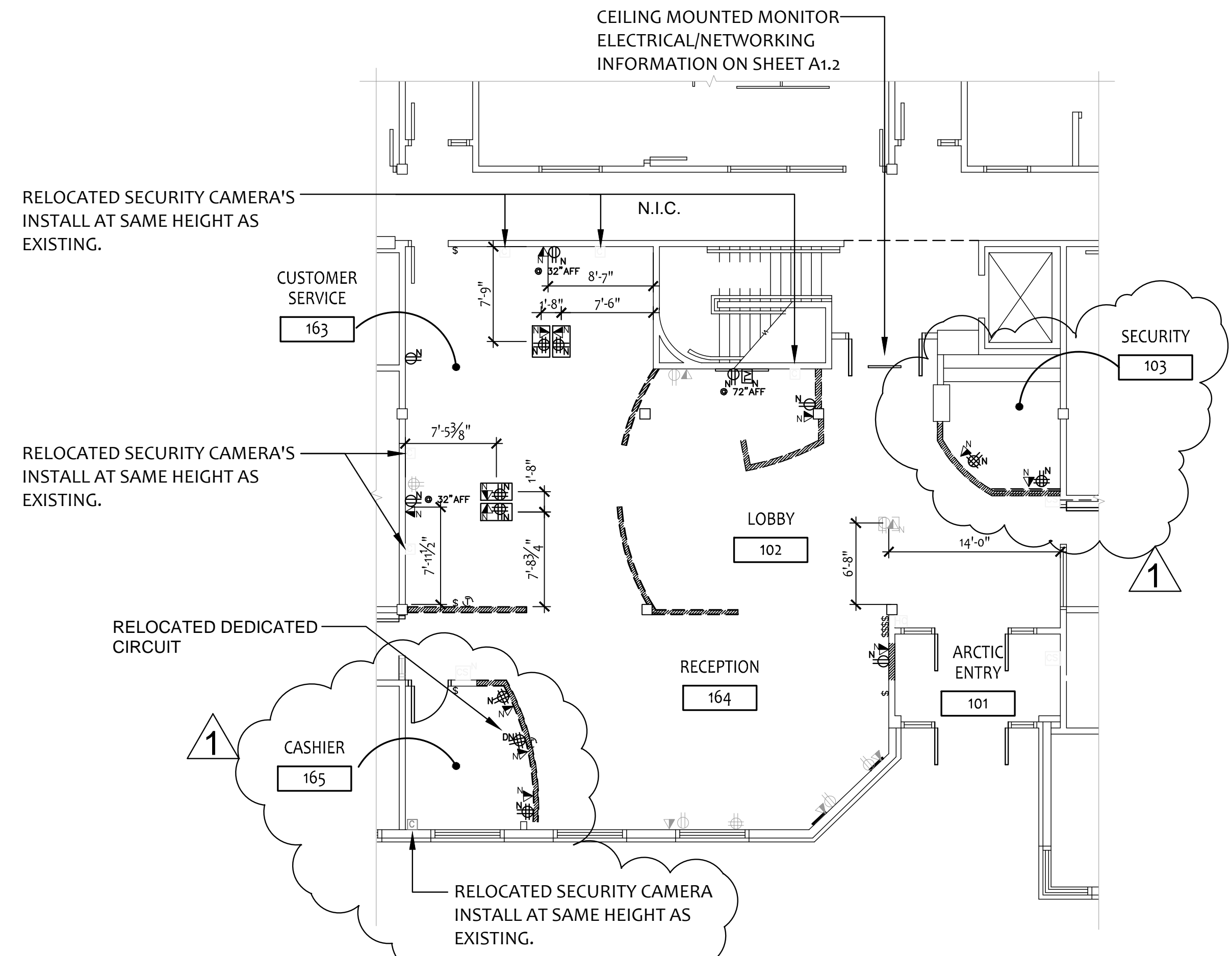
ELECTRICAL PLAN - NEW
