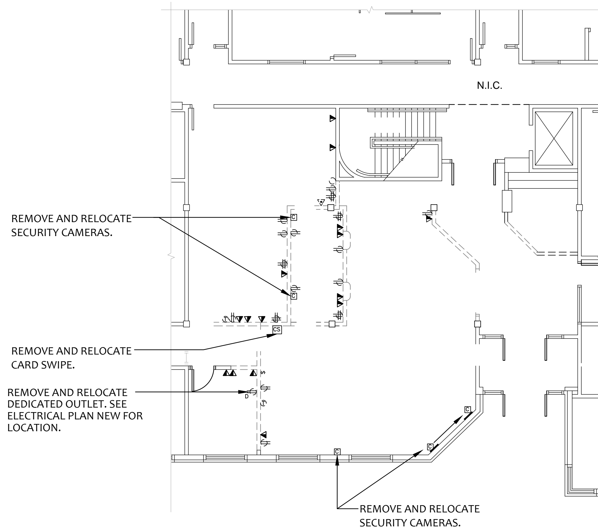
ELECTRICAL PLAN - DEMOLITION
