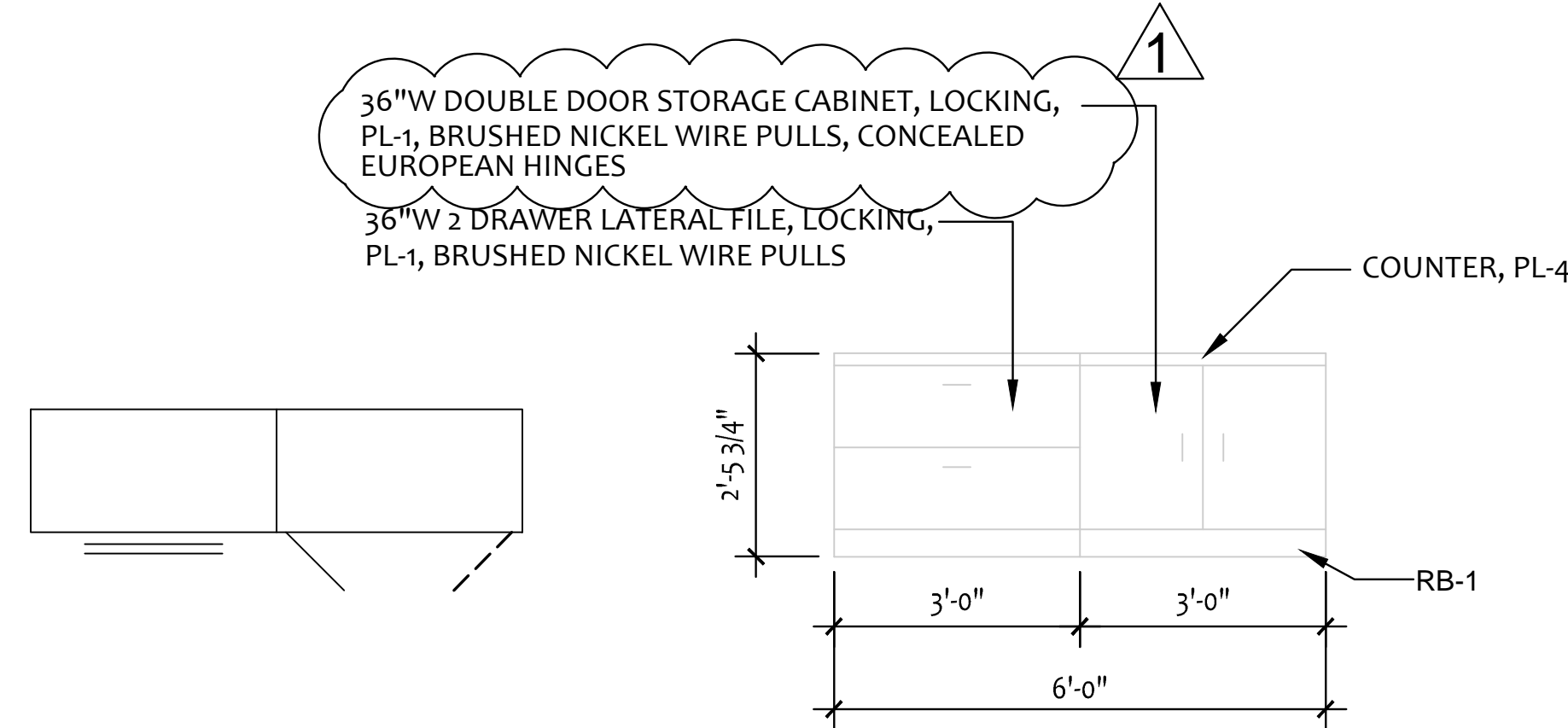
6 CUSTOMER SERVICE STORAGE 1/2"=1'-0"
