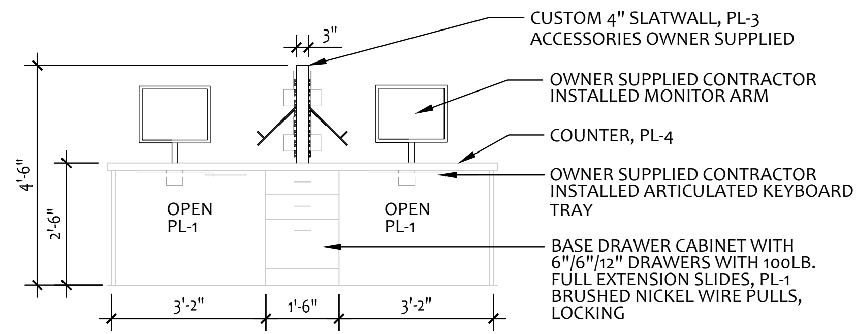
1 CUSTOMER SERVICE DESK - ELEVATION 1/2"=1'-0"
