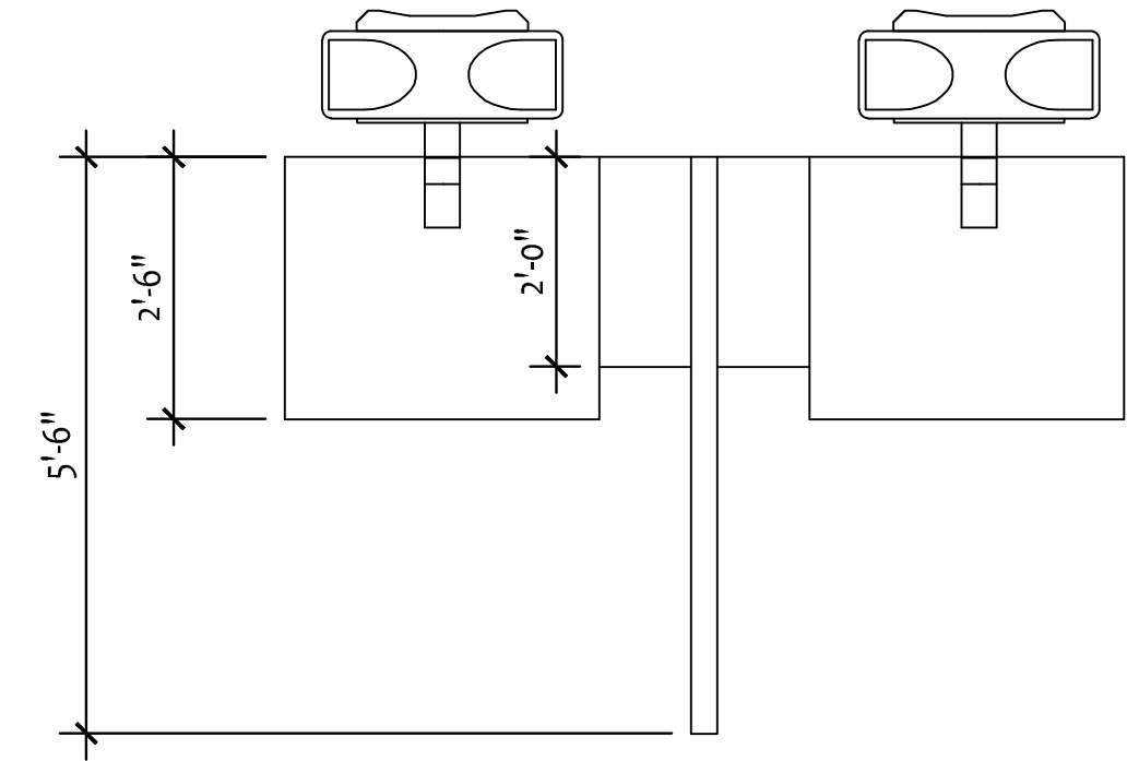
5 CUSTOMER SERVICE DESK - PLAN VIEW 1/2"=1'-0"
