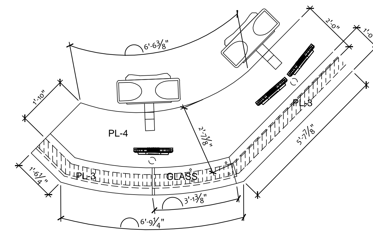
16 SECURITY STATION - PLAN VIEW 1/2"=1'-0"
