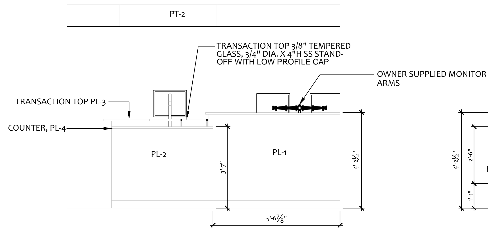
15 SECURITY STATION 1/2"=1'-0"
