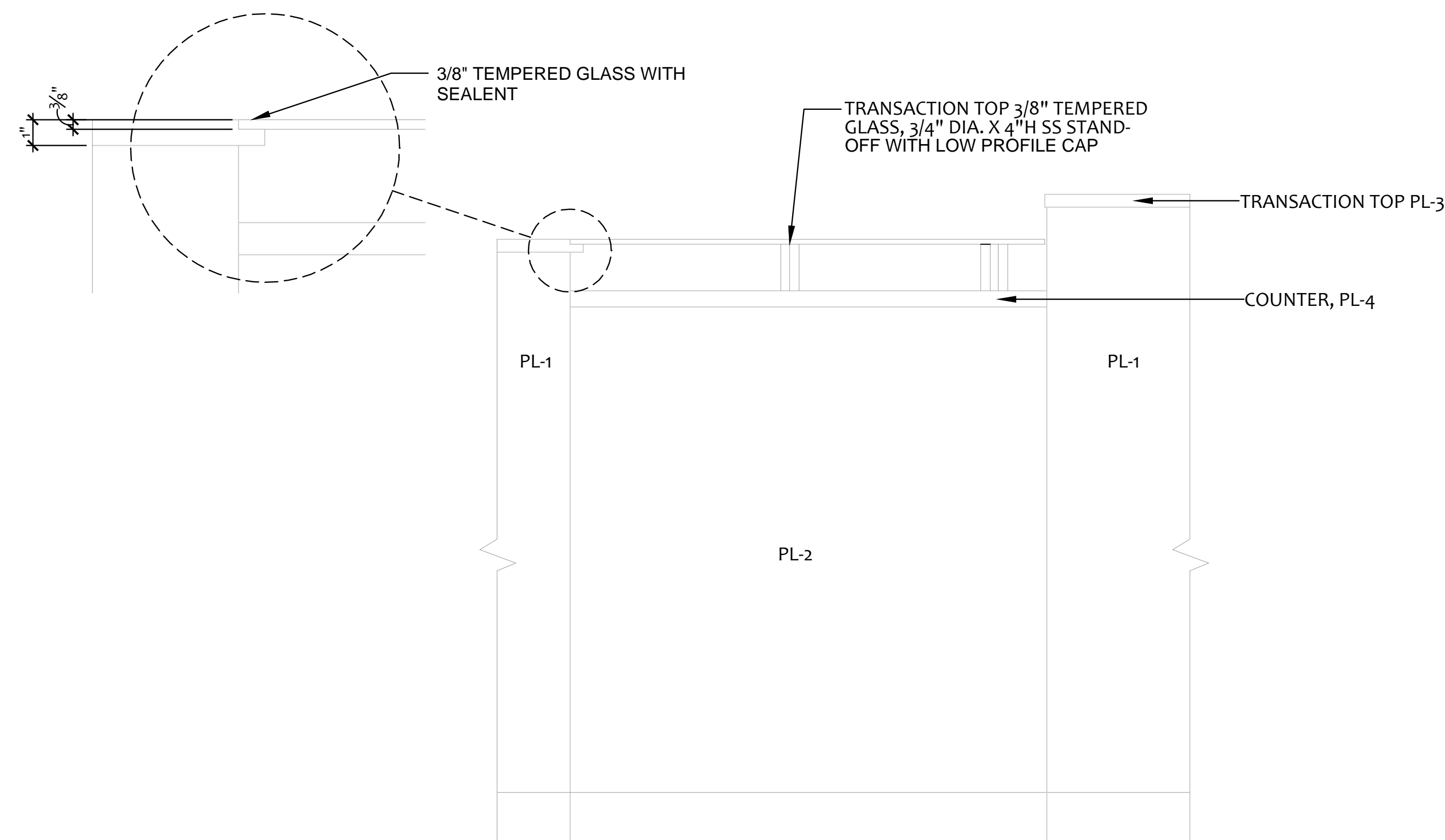
17 SECURITY STATION - TRANSACTION TOP DETAIL 1-1/2"=1'-0"
